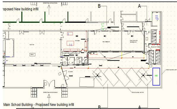
Part general arrangement layout plan
